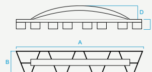
PIALLA IN METALLO
